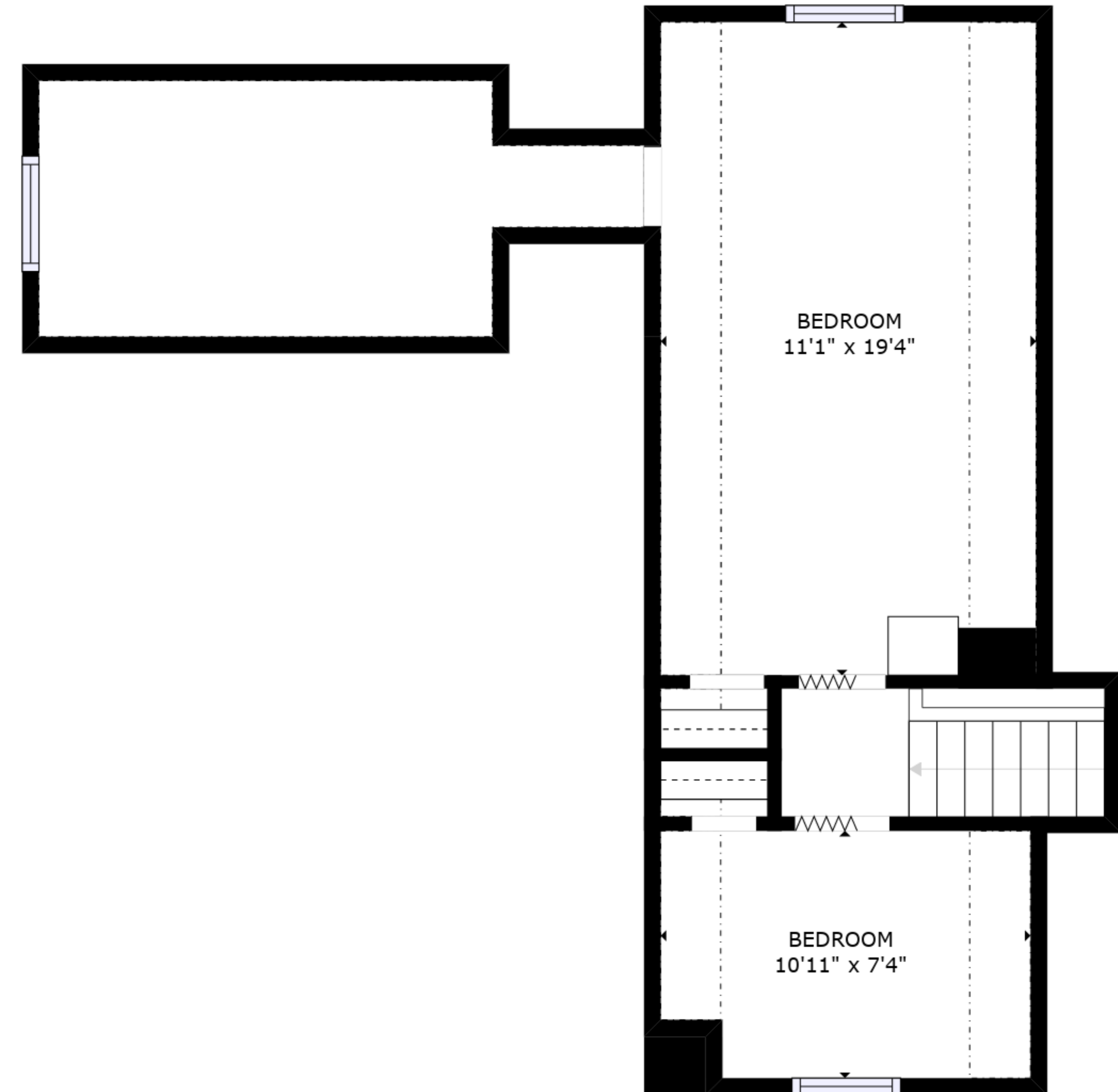
FLOOR 2
