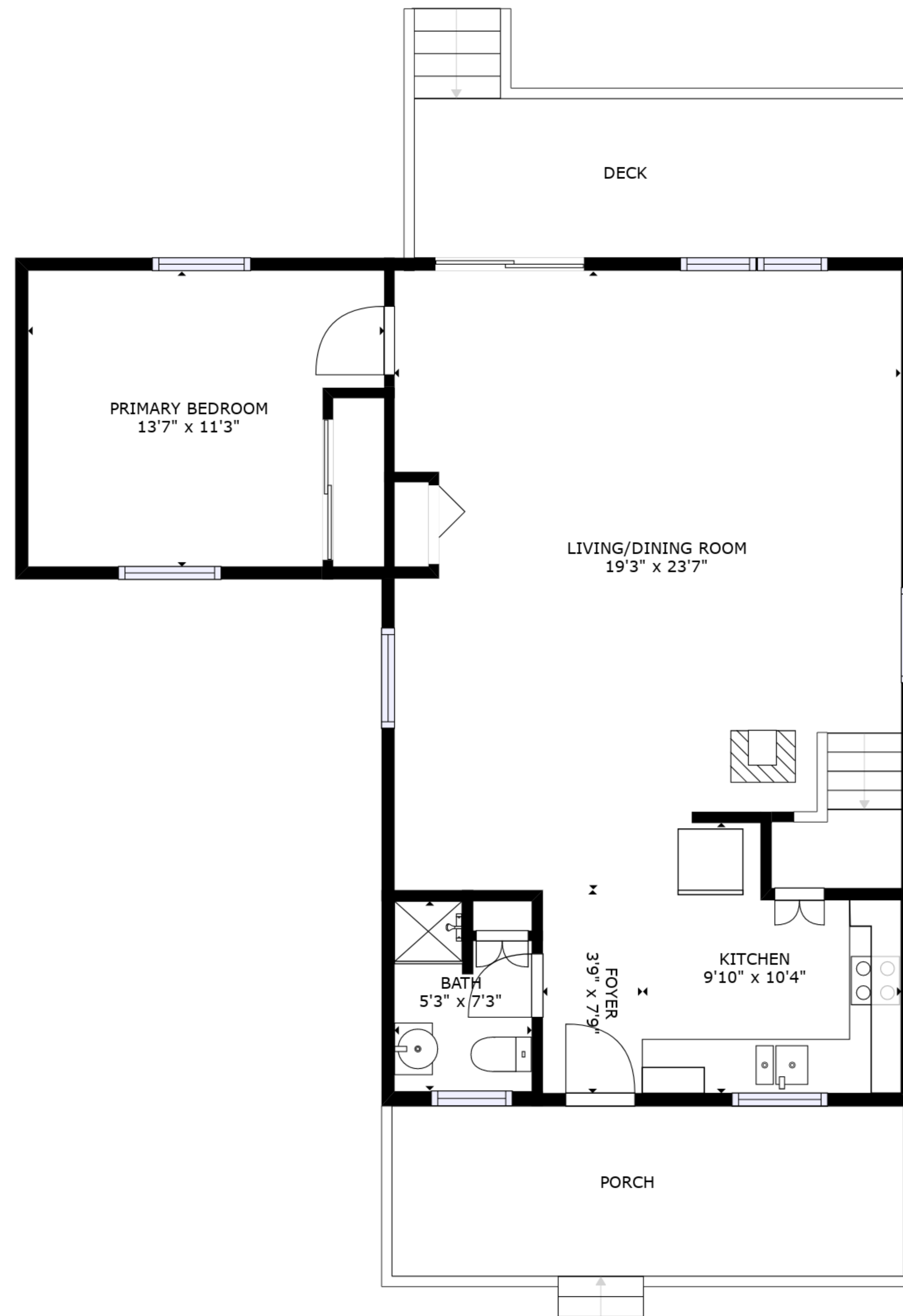
FLOOR 1
