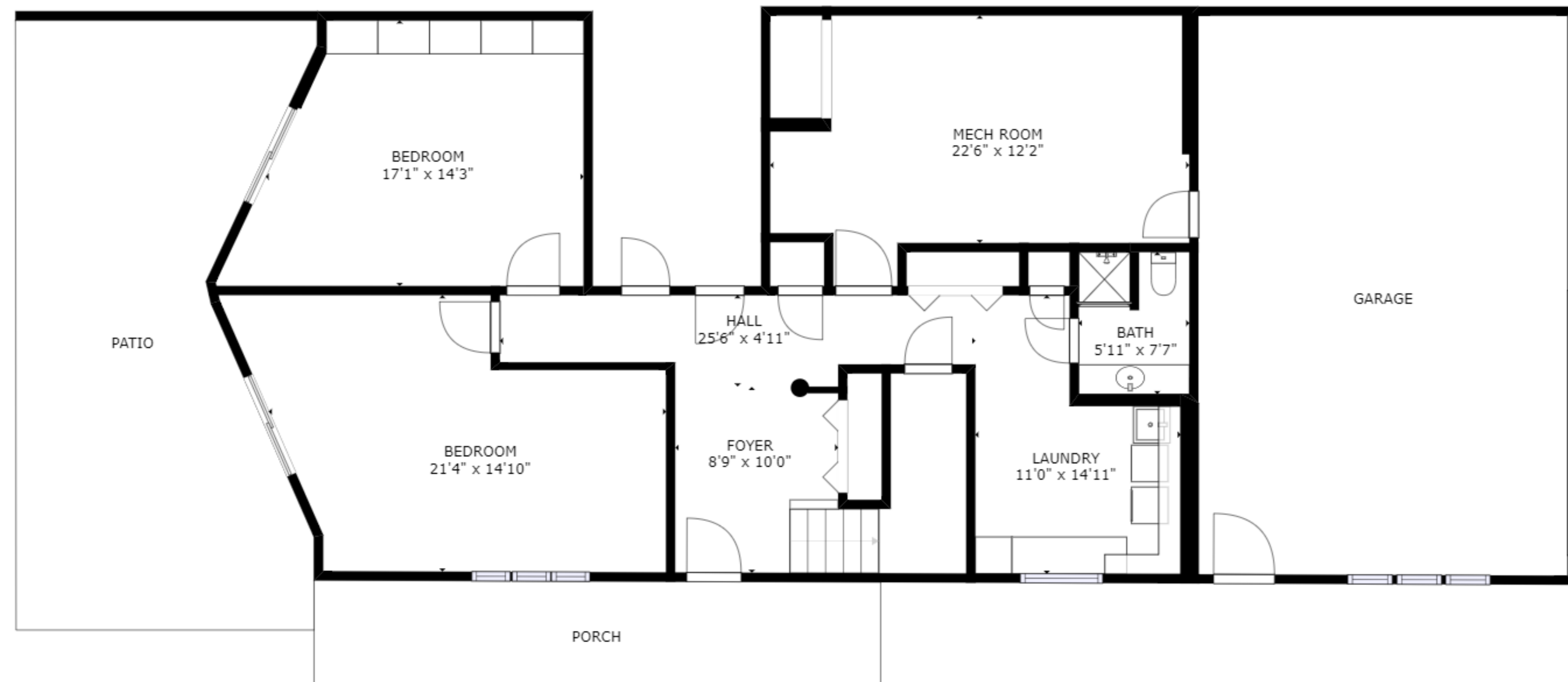
FLOOR 1
