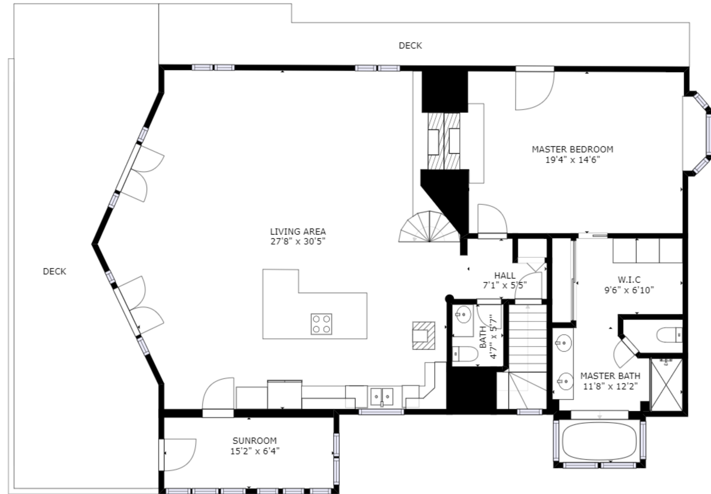
FLOOR 2
